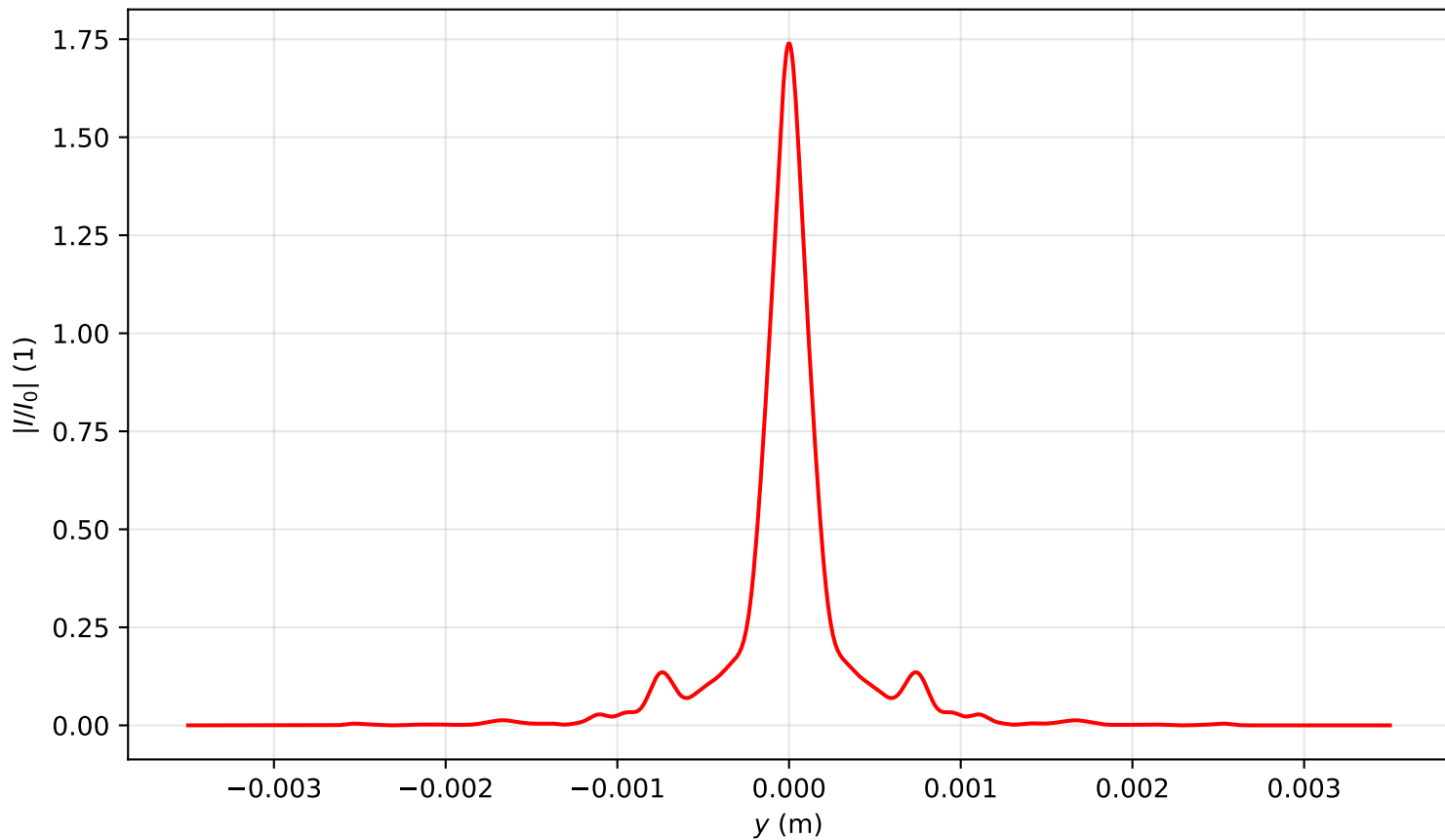
Intensity profile I(x=0, y, z=1.433)/I_0 , P_{in}=7.0P_{cr} , artificial time
